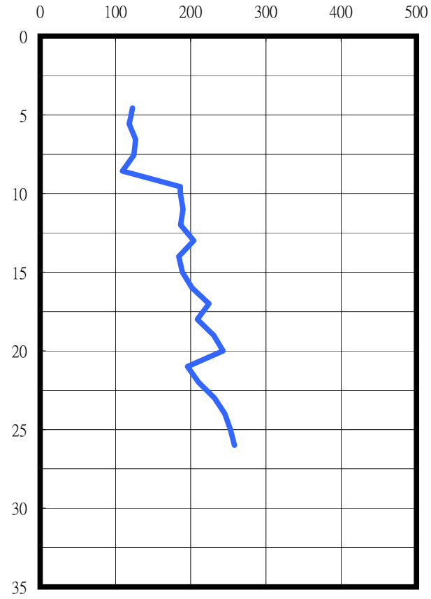
S-Wave
