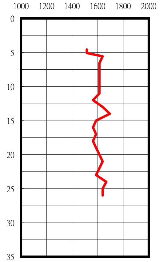
P-Wave
