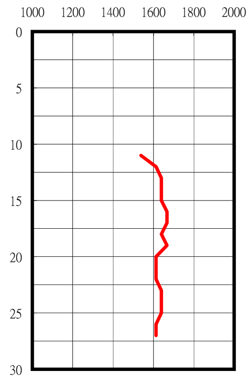
P-Wave
