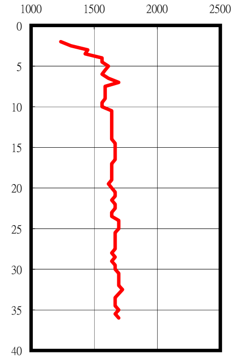
P-Wave (m/sec)
