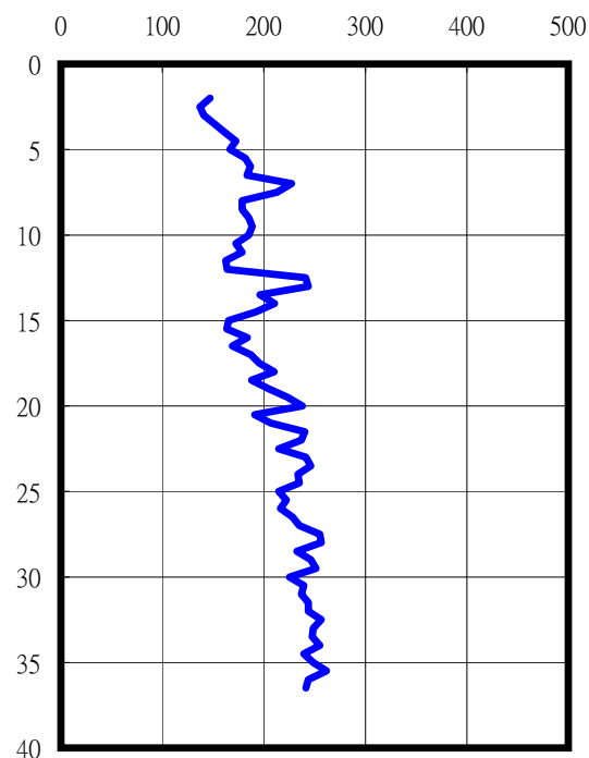
S-Wave (m/sec)
