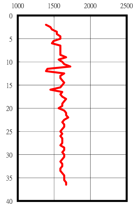
P-Wave (m/sec)
