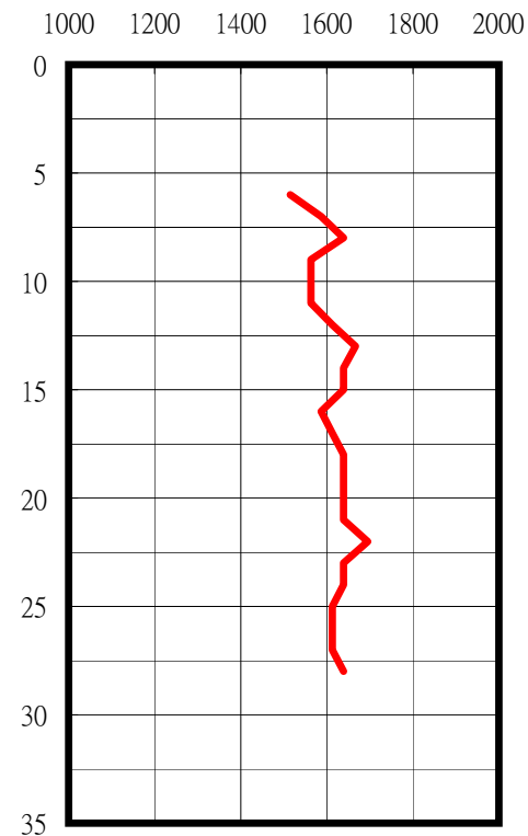
P-Wave
