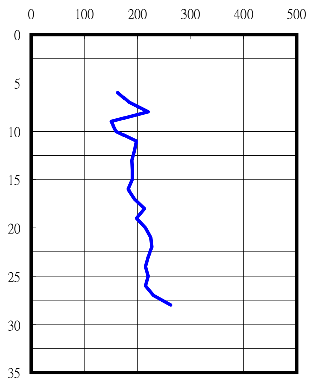
S-Wave
