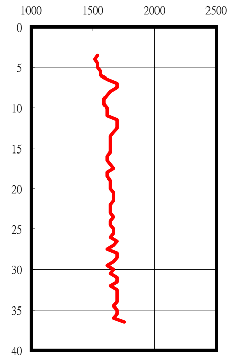
P-Wave (m/sec)
