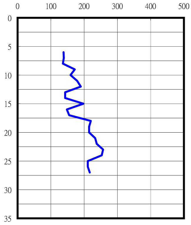
S-Wave
