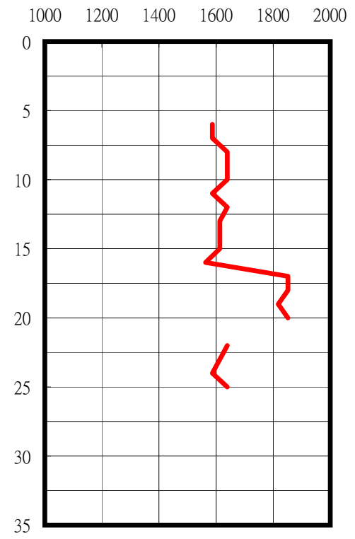
P-Wave
