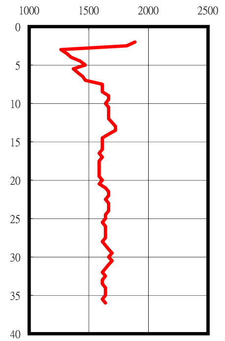
P-Wave (m/sec)
