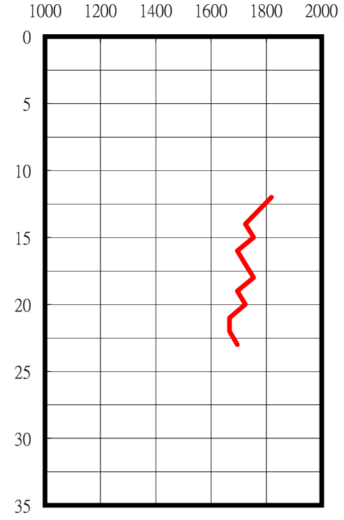
P-Wave
