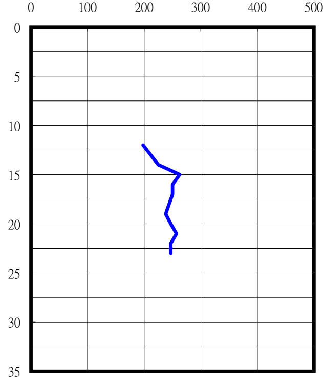
S-Wave
