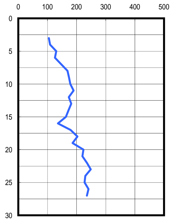
S-Wave
