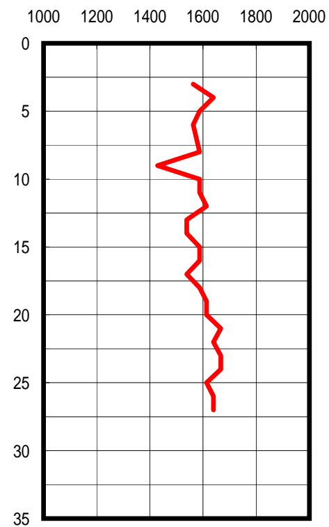
P-Wave
