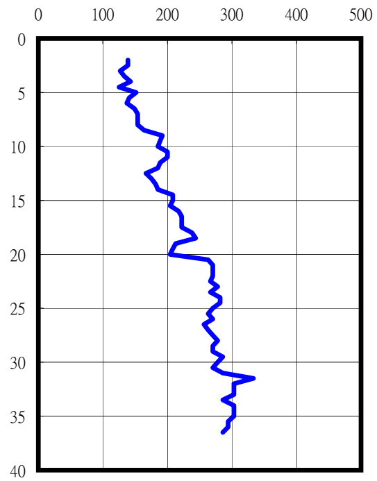
S-Wave (m/sec)
