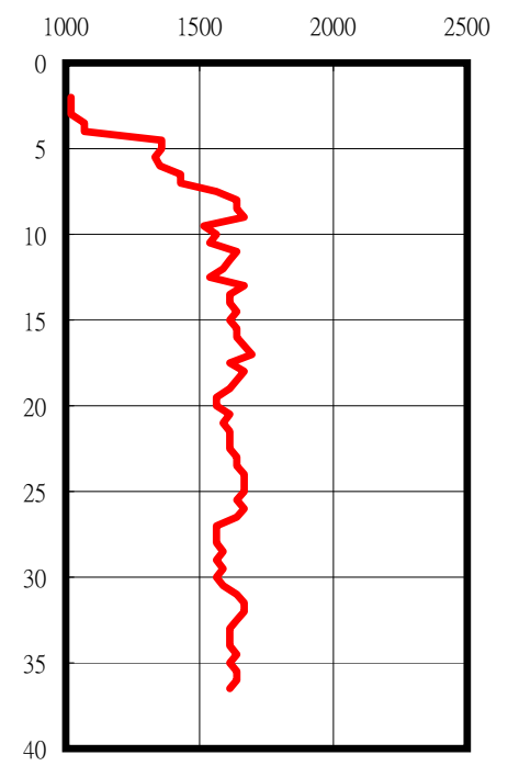
P-Wave (m/sec)
