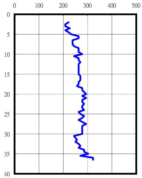
S-Wave (m/sec)
