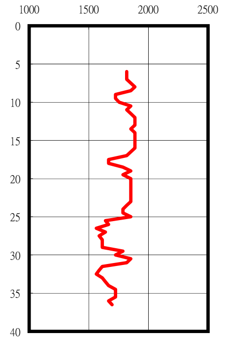
P-Wave (m/sec)
