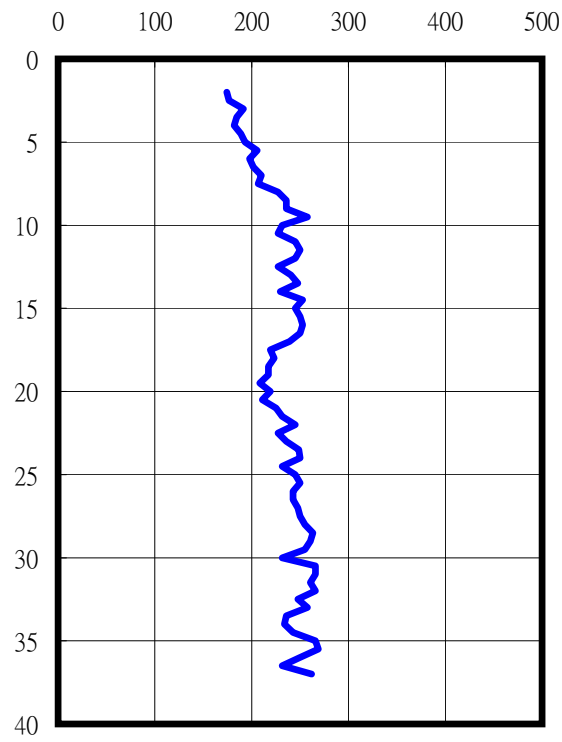
S-Wave (m/sec)
