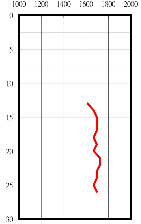
P-Wave
