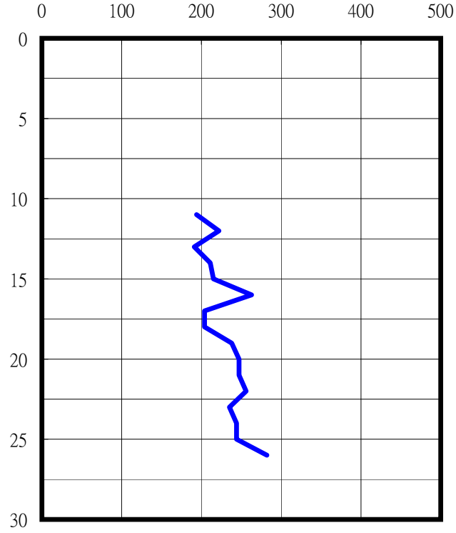
S-Wave
