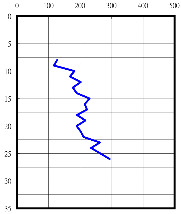
S-Wave
