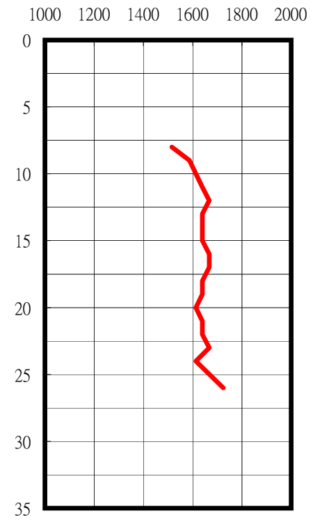
P-Wave
