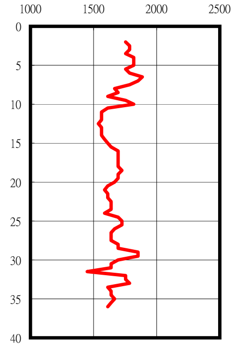
P-Wave (m/sec)
