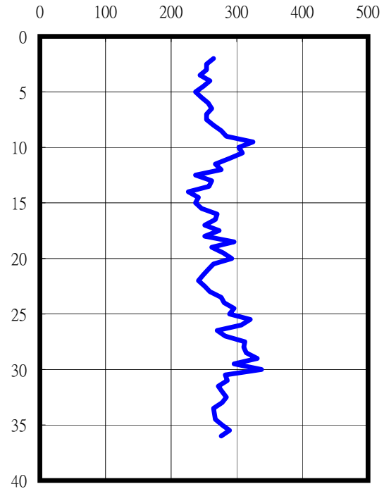
S-Wave (m/sec)
