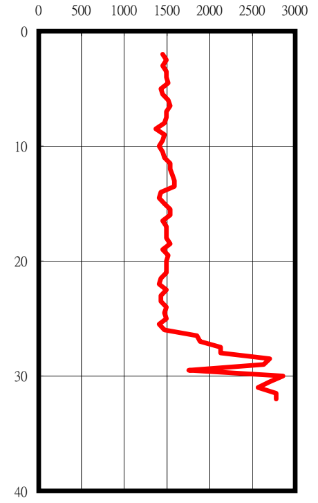
P-Wave (m/sec)
