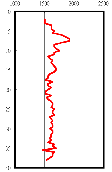
P-Wave (m/sec)
