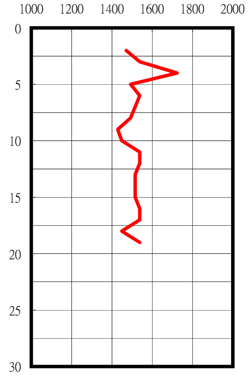
P-Wave
