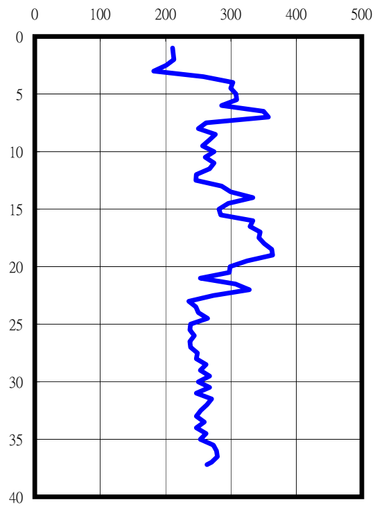
S-Wave (m/sec)
