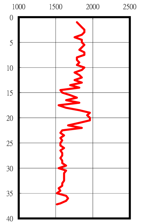
P-Wave (m/sec)
