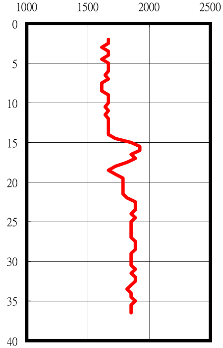
P-Wave (m/sec)
