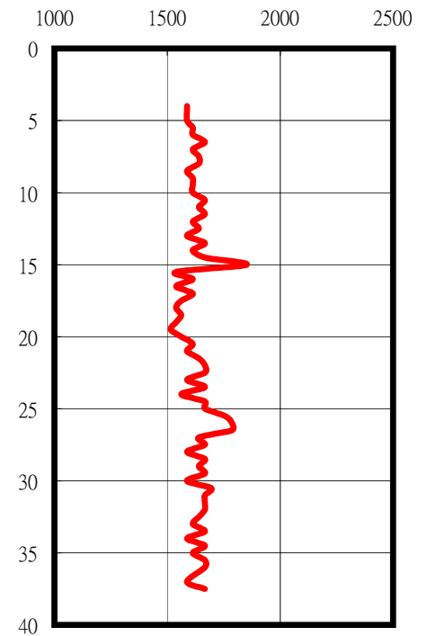
P-Wave (m/sec)
