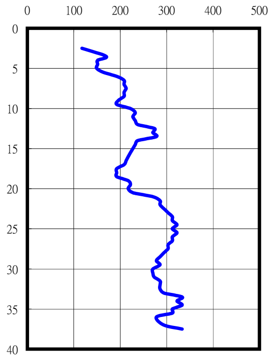
S-Wave (m/sec)
