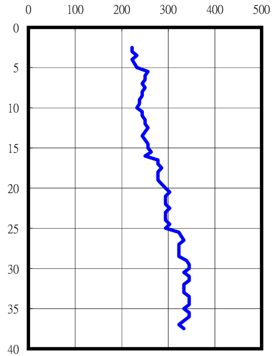
S-Wave (m/sec)
