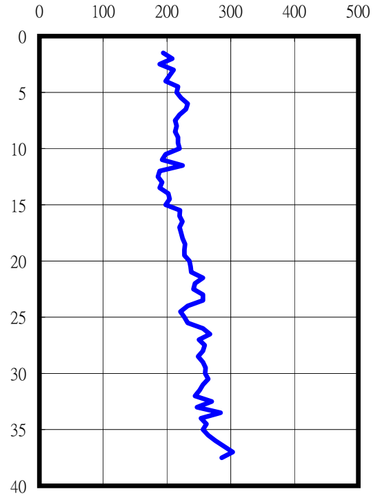
S-Wave (m/sec)
