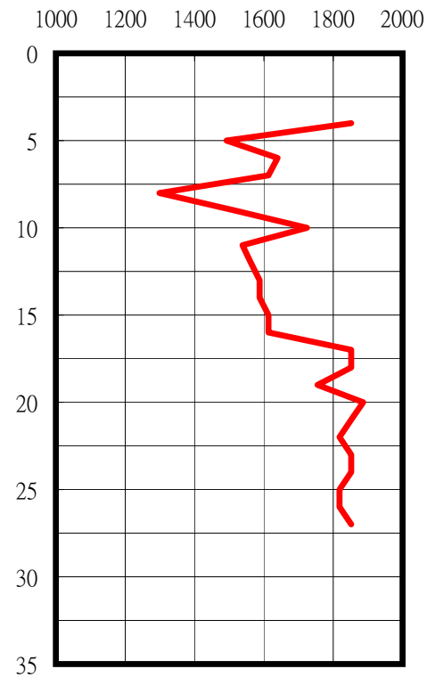
P-Wave
