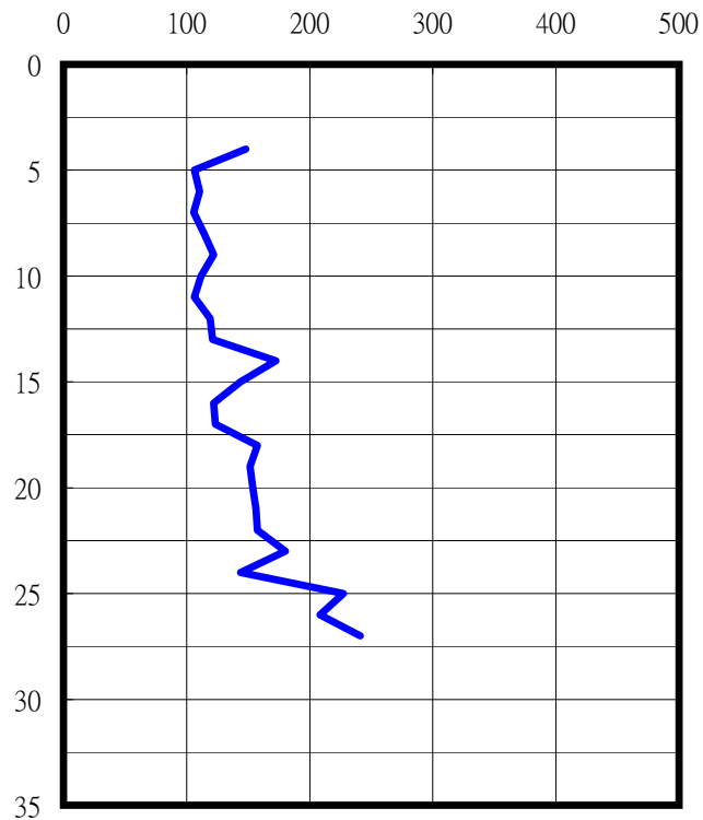
S-Wave
