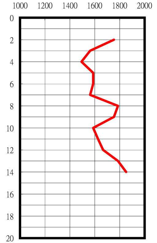
P-Wave
