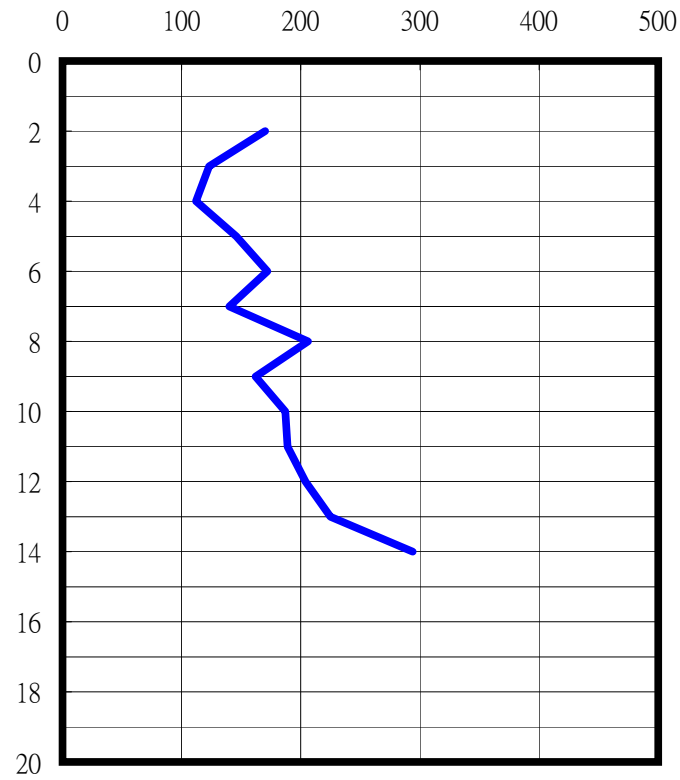
S-Wave
