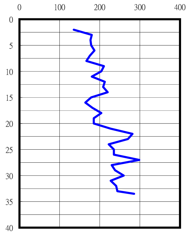
S-Wave
