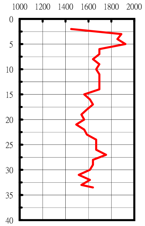
P-Wave
