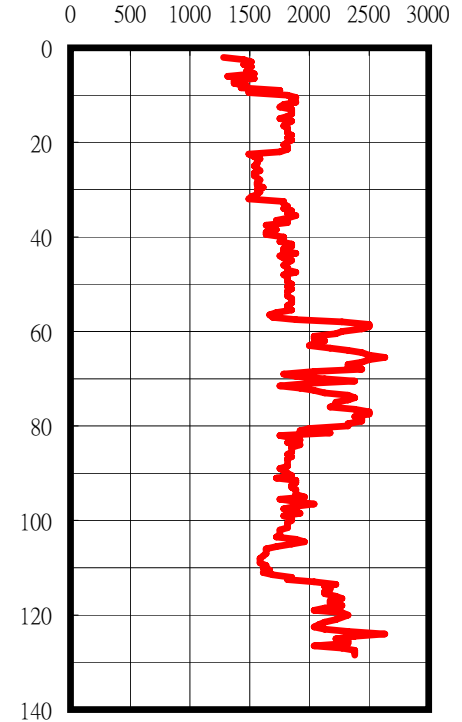
P-Wave (m/sec)
