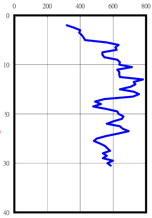
S-Wave (m/sec)
